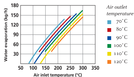
VSD-50 co-current atomization
