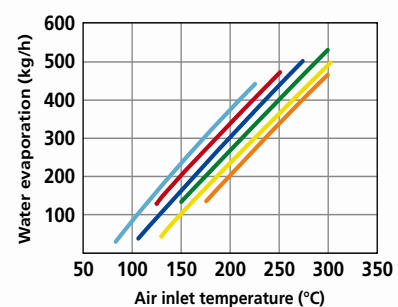
VSD-80 co-current atomization
