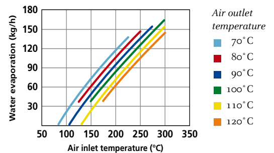
VSD-50 co-current atomization
